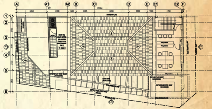
Lower Roof Plan (future Attic) Scale : NTS
