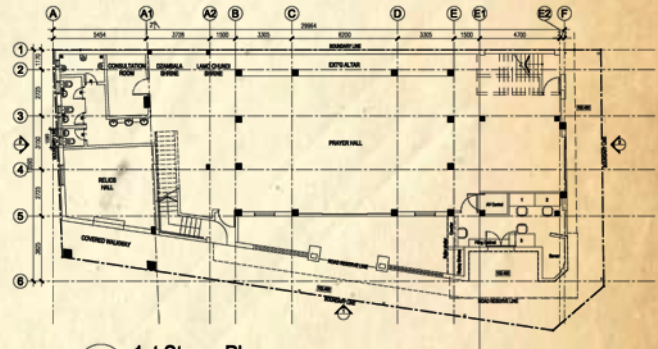
1st Storey Plan Scale : NTS
